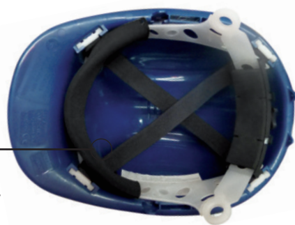
TEXTILE SUSPENSION WITH TIGHTENING SCREW 80529-SR
